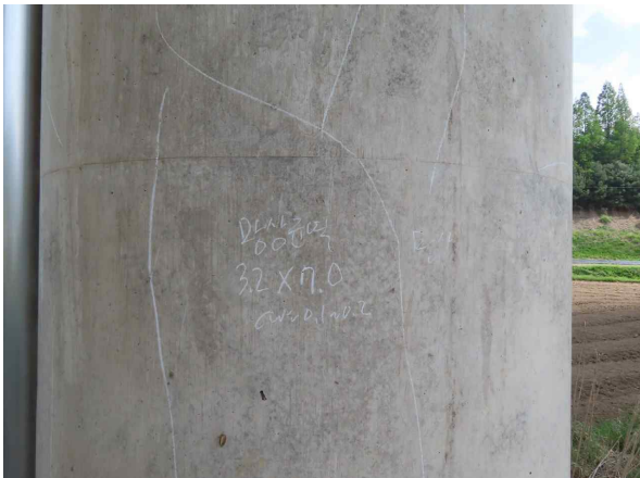
P3 교각 망상균열 (7.0m×3.2m, Cw=0.1~0.2mm)
