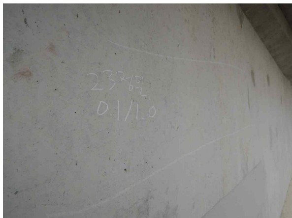
거더 S3-G9 균열 (0.1mm/1.0m, 2EA)
